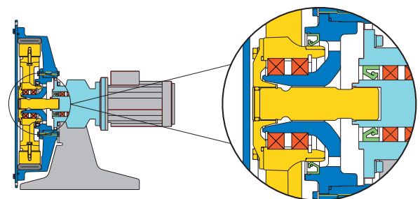
Bredel direct-coupled
